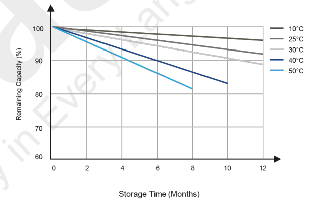
Temperature on Self Discharge Curve
